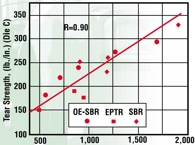
Plot of ASTM Die C Tear Strength as a Function of Stress at 300% Elongation
