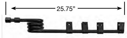
Straight HD Round Triple Coil
